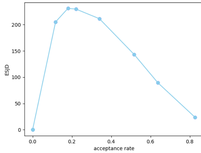
Figure 9: Relation of ESJD and acceptance rate for section 4.5.2
