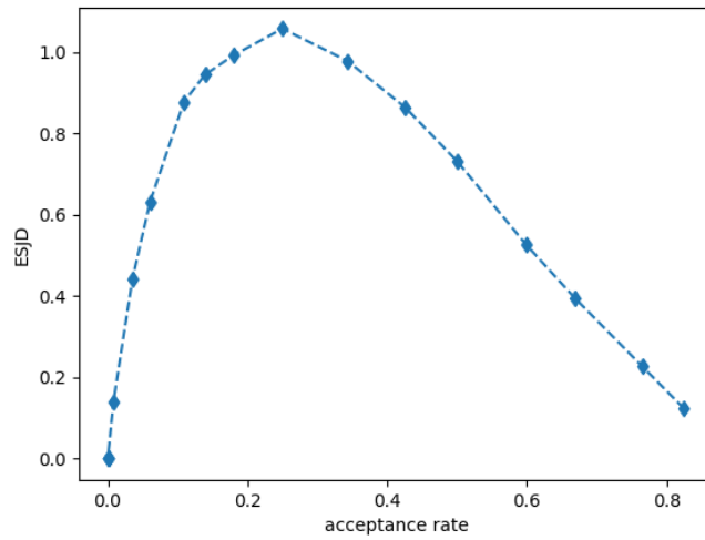
Figure 2: Relation of ESJD and acceptance rate with homogeneous proposed distribution containing known scaling factors.
