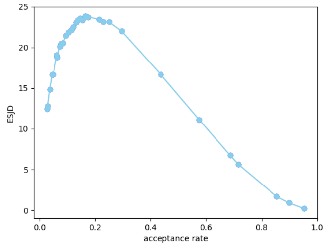
Figure 8: Relation of ESJD and acceptance rate for section 4.5.1
