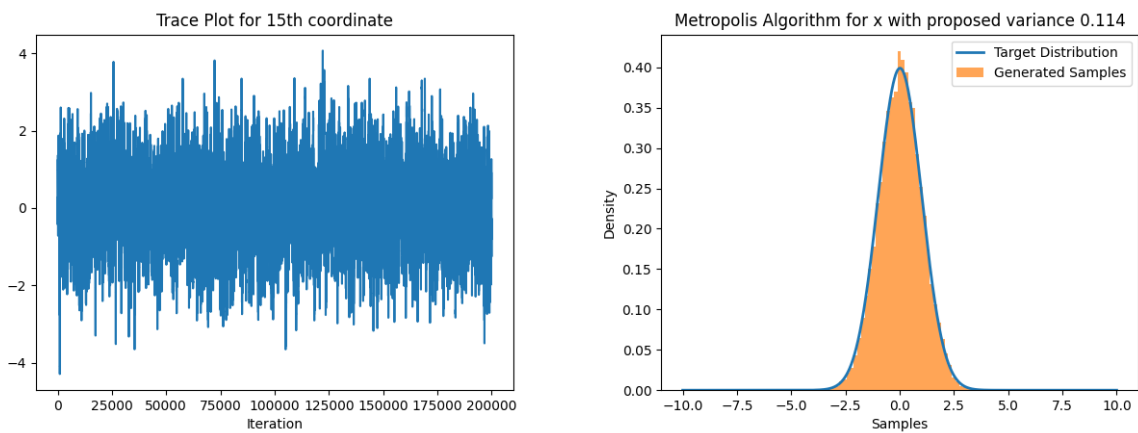
Figure 5: Trace plot and histogram of 15th coordinate for section 3.2.2
