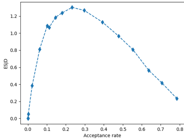
Figure 4: relation of ESJD and acceptance rate for section 3.2.2
