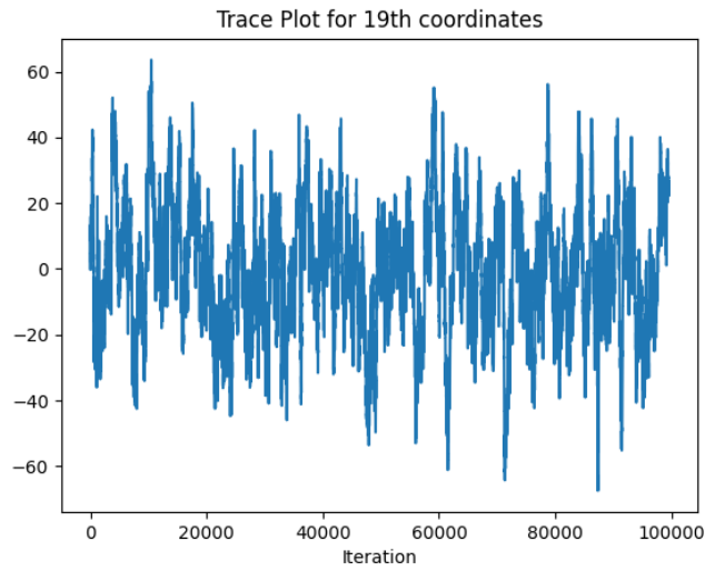
Figure 7: Trace plot of the 19th coordinate for section 4.5.1
