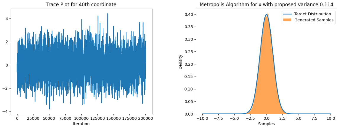
Figure 6: Trace plot and histogram of 40th coordinate for section 3.2.2
