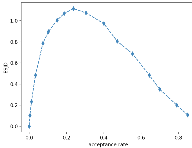
Figure 3: Relation of ESJD and acceptance rate with inhomogeneous proposed distribution containing known scaling factors.
